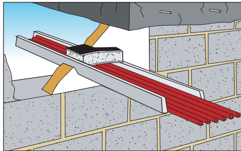
PFC Corofil Coated Panel System fitted around cable tray in compartment wall. PFC Corofil C25 Cable Firestop compressed into the interior of cable tray
