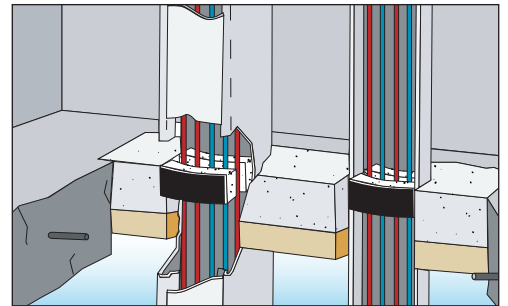
PFC Corofil C25 Cable Firestop filling electrical trunking and cable trays where they pass through compartment floors. PFC Corofil Firestop Compound making good service riser
