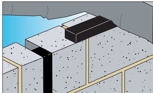
PFC Corofil C500X compressed into blockwork joints
