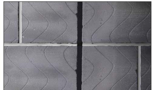
PFC Corofil C500X firestopping vertical expansion joint
